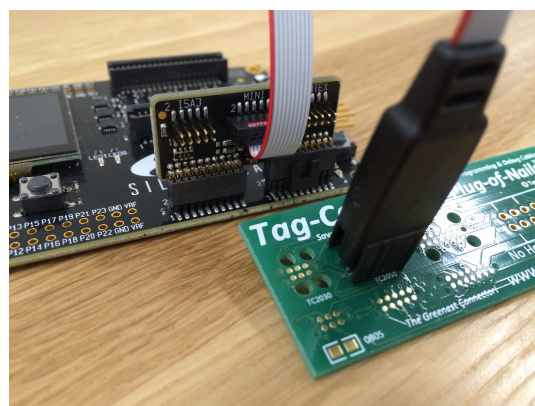
Figure 5.5. TC2050-IDC-050-ALL Cable
