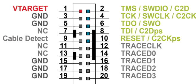
Figure 3.6. Debug Connector
