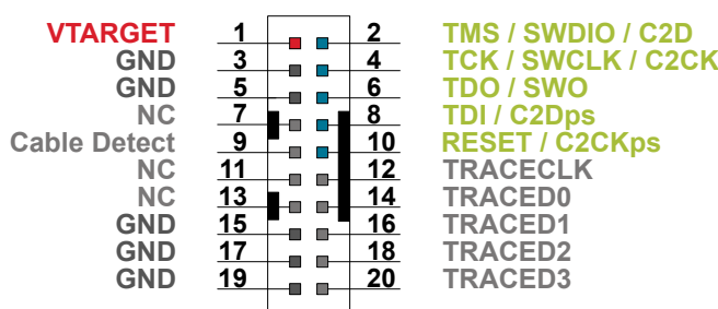
Figure 3.6. Debug Connector
