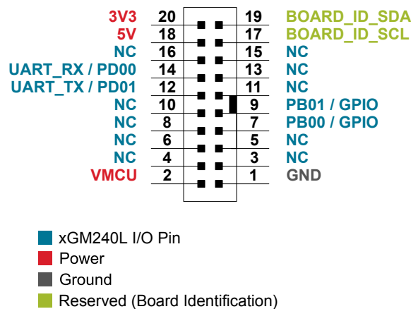
Figure 3.5. EXP Header
