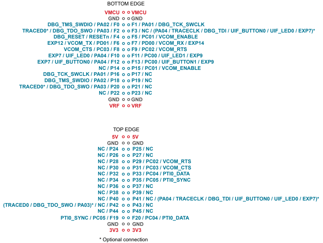
Figure 3.3. Wireless Pro Kit Mainboard (BRD4002A) Breakout Pad Pin Mapping
